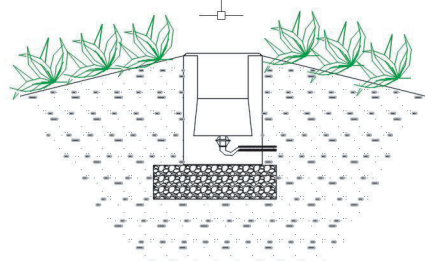
Incorrect Fixing method Do not install on hollow areas
