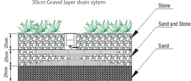
Correct Fixing Method Install on raised areas
