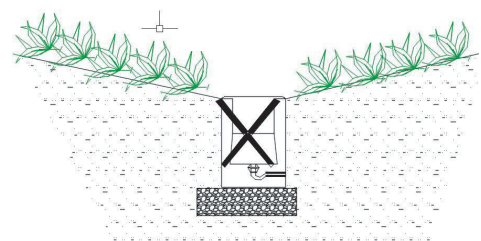
Incorrect Fixing method Do not install on hollow areas
